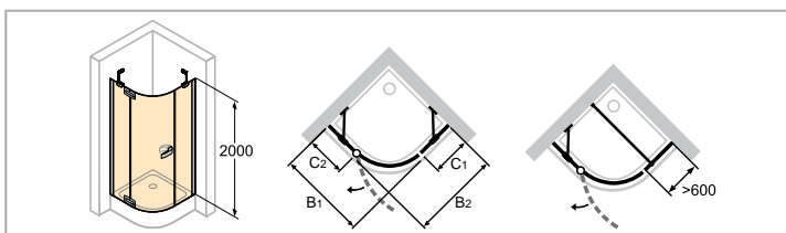
Left-hand fixing
