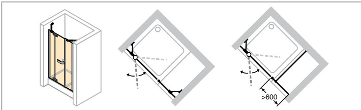
Left-hand fixing
