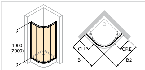
Acrylic version
