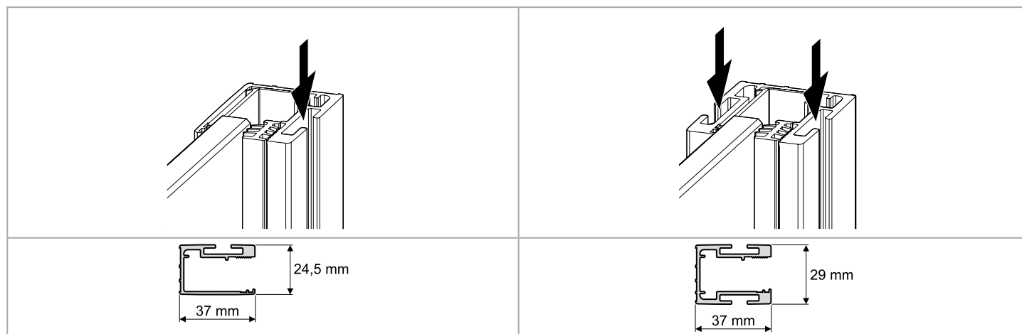
Select+ kit profile
