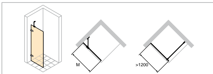
Left-hand fixing
