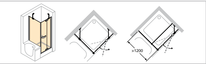
Right-hand fixing
