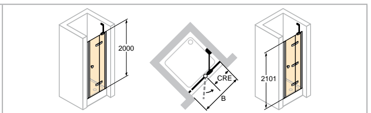
Right-hand fixing
