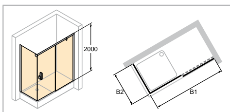
Right-hand fixing
