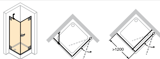
Right-hand fixing
