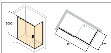
Left-hand fixing
