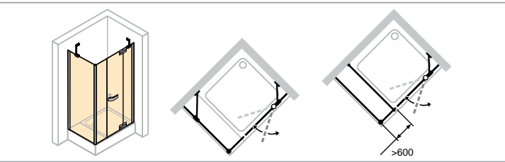
Right-hand fixing
