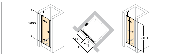
Left-hand fixing
