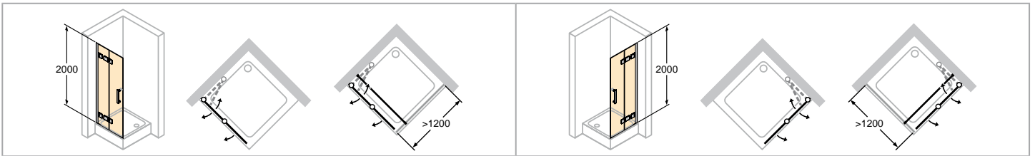
Left-hand fixing
