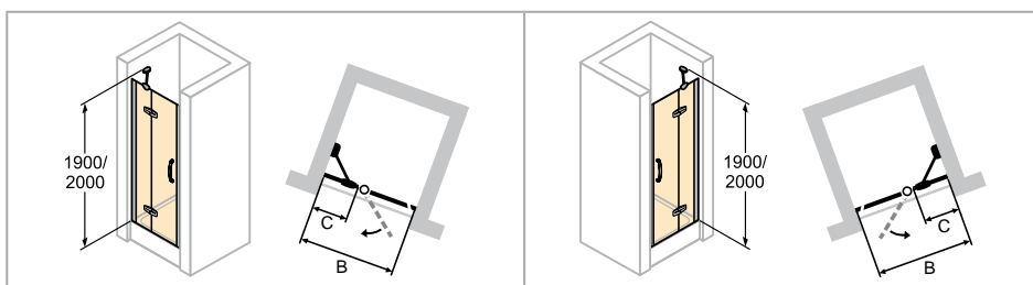
Left-hand fixing
