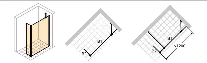
Right-hand fixing
