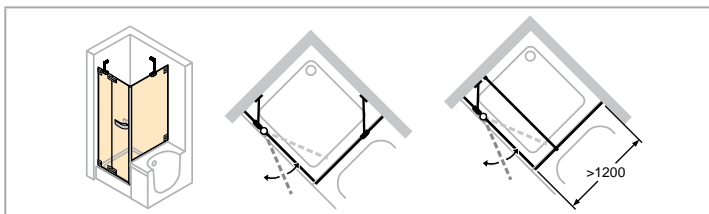
Left-hand fixing
