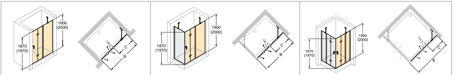
SFTN with fixed segment = SFT with fixed segment + supplement set
