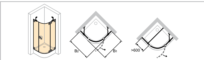
Right-hand fixing
