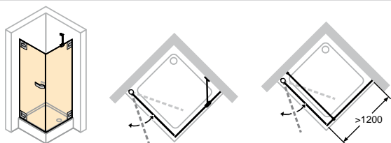
Left-hand fixing
