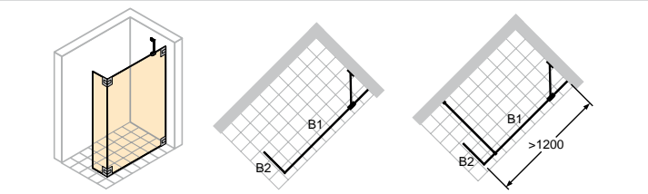
Right-hand fixing
