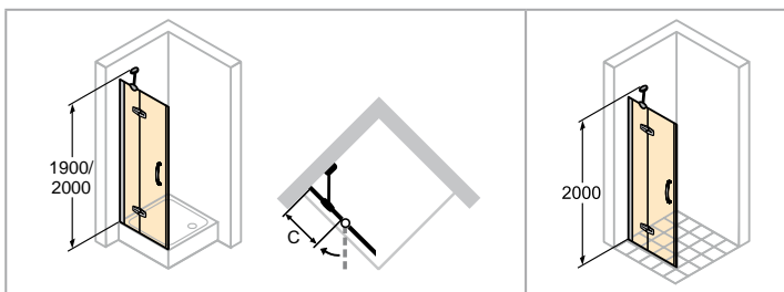
Left-hand fixing
