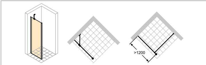
Left-hand fixing
