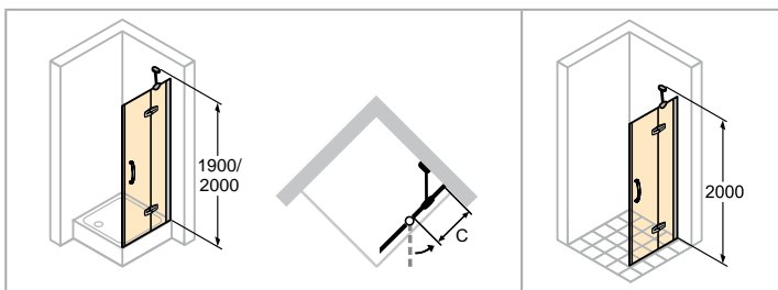
Right-hand fixing
