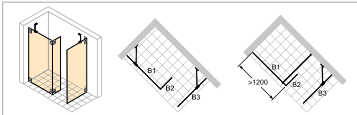
Left-hand fixing
